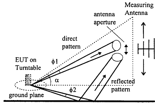
Figure 1. EUT measured on an OATS
