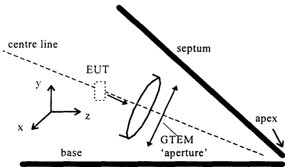
Figure 3. EUT measured in a GTEM
