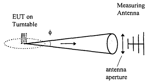
Figure 2. EUT measured in a Fully Anechoic Room
